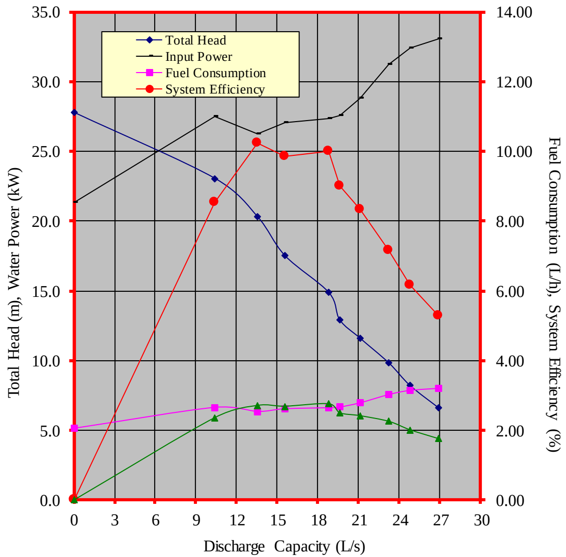
Figure 2. Performance characteristic curves of the KATO KSP40 centrifugal pump coupled to KATO KD120-N diesel engine
